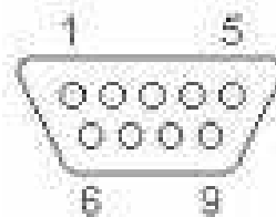
DB9 Male Front View
