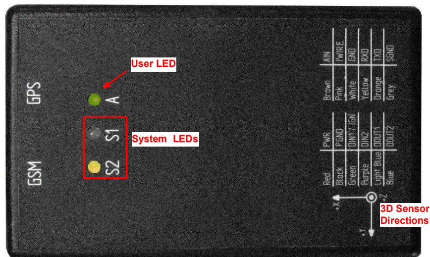
Top-side view
