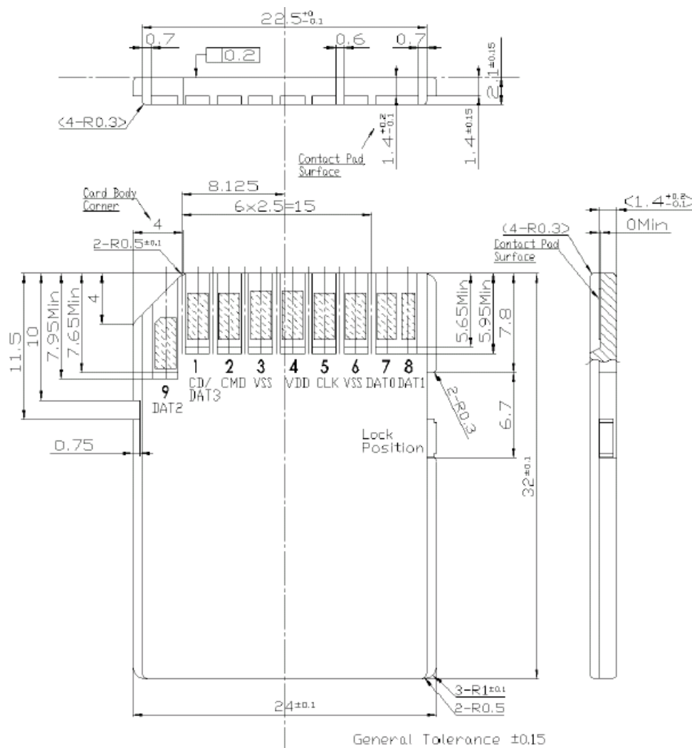
Figure 2-11: Physical Dimension
