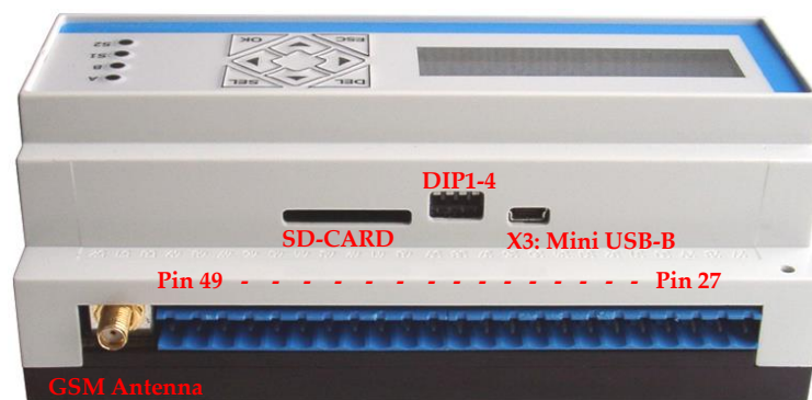
Top-side view
