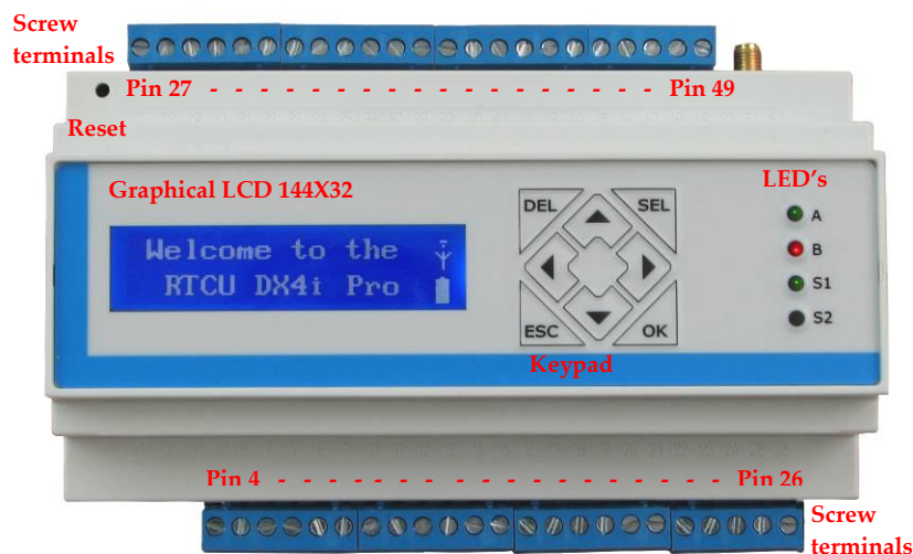
Front view with pluggable screw terminals.
