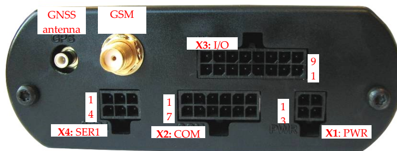
Back-side view
